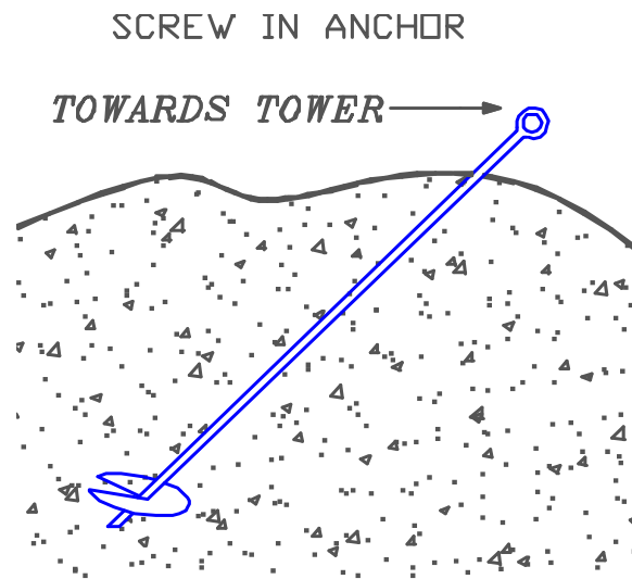
Picture B-1: Installing Screw-in Anchors
