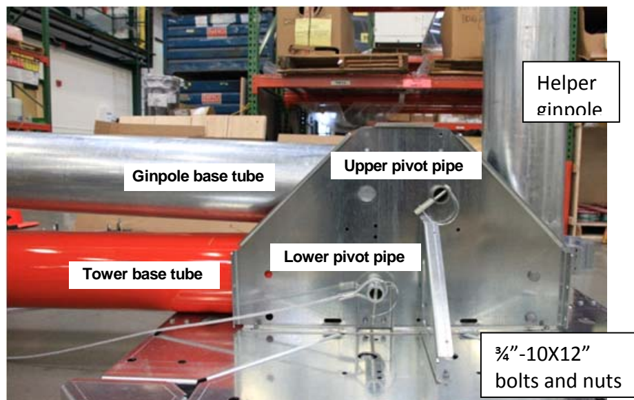
Picture 3-63: Complete baseplate and tower assembly ready for raising
