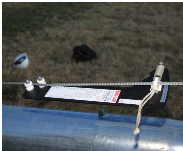
Picture 3- 80: Correct use of tension gauge
