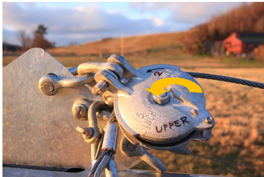
Picture 3-73: Reeving through pulley #2
