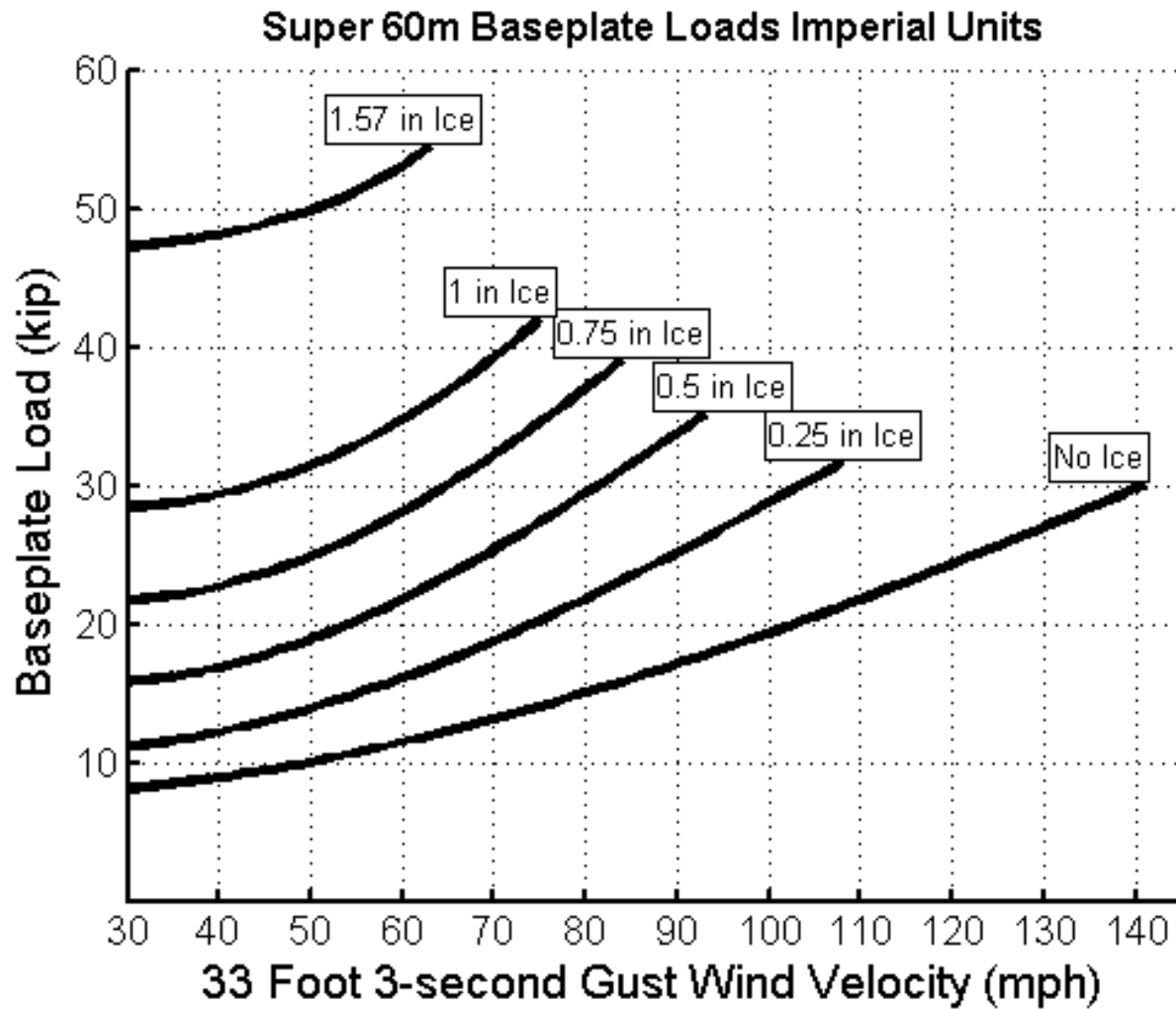
Picture A-8: Super 60m Maximum Baseplate Loads Imperial Units
